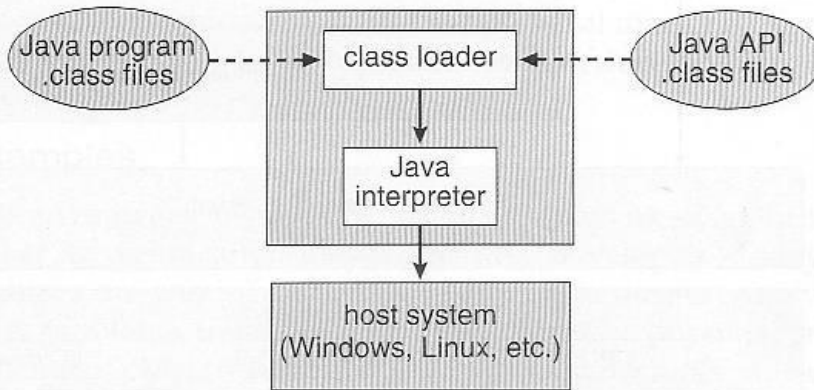
Figure 2.20 The JVM
