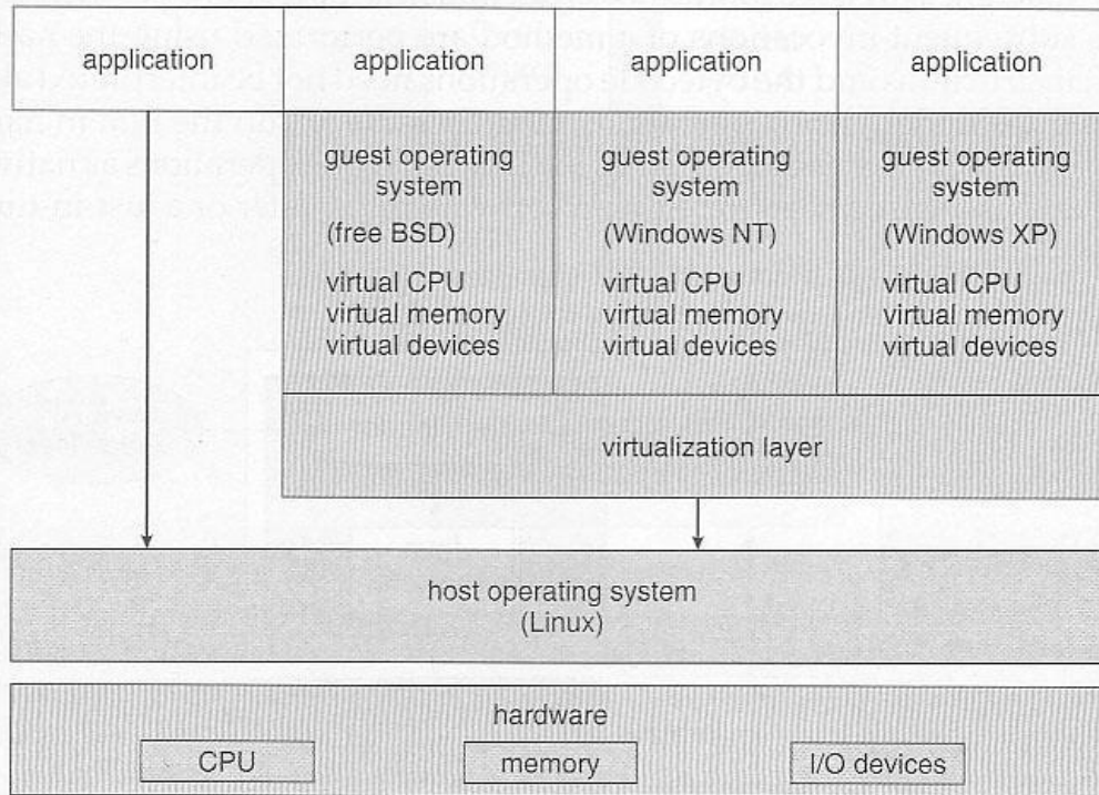
Figure 2.19 VMware architecture
