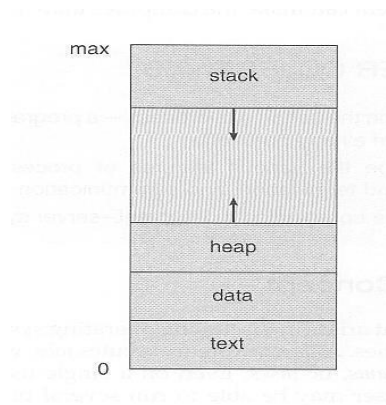
Figure 3.1 Process in memory.
