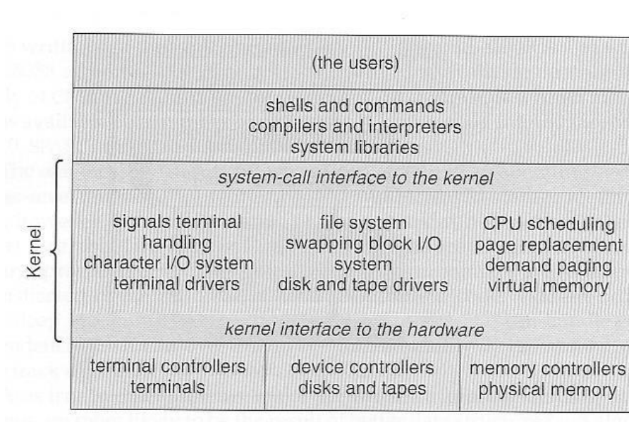
Figure 2.13 UNIX System Structure
