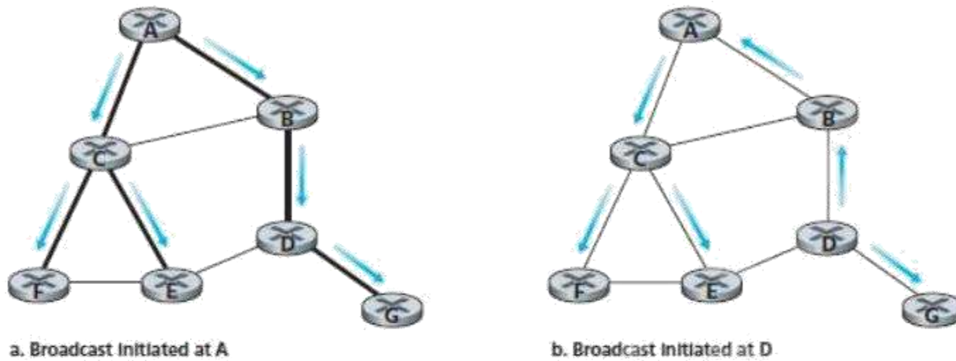
Figure 3.33: Broadcast along a spanning-tree
