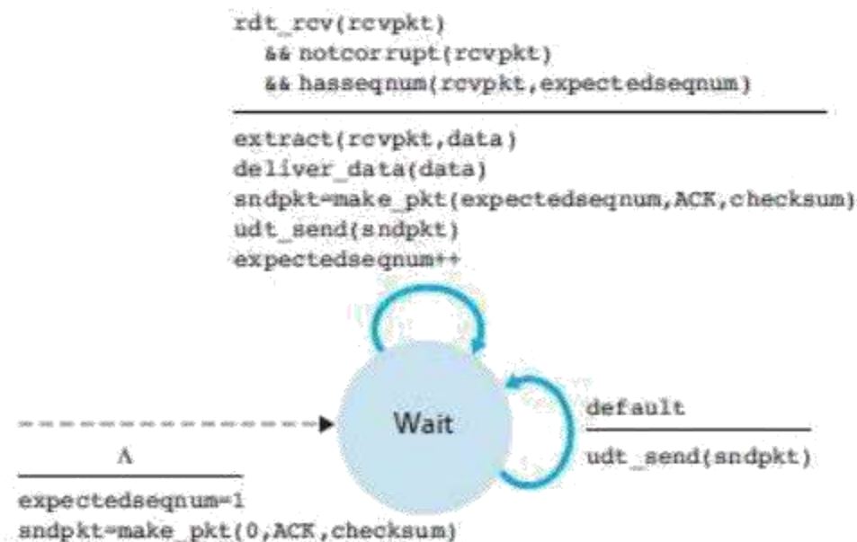
Figure 2.19: Extended FSM description of GBN receiver
