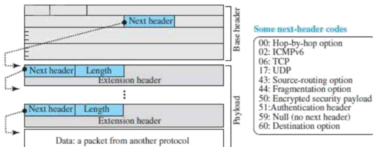
Figure 3.19: Payload in IPv6 datagram
