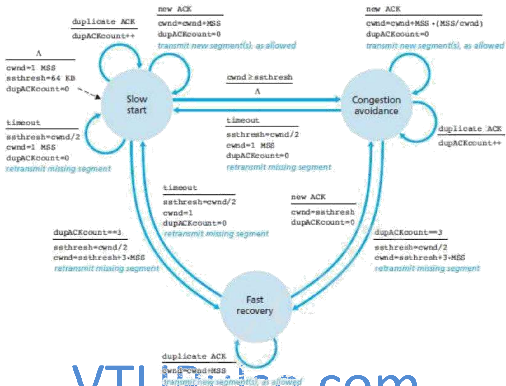
Figure 2.43: FSM description of TCP congestion-control
