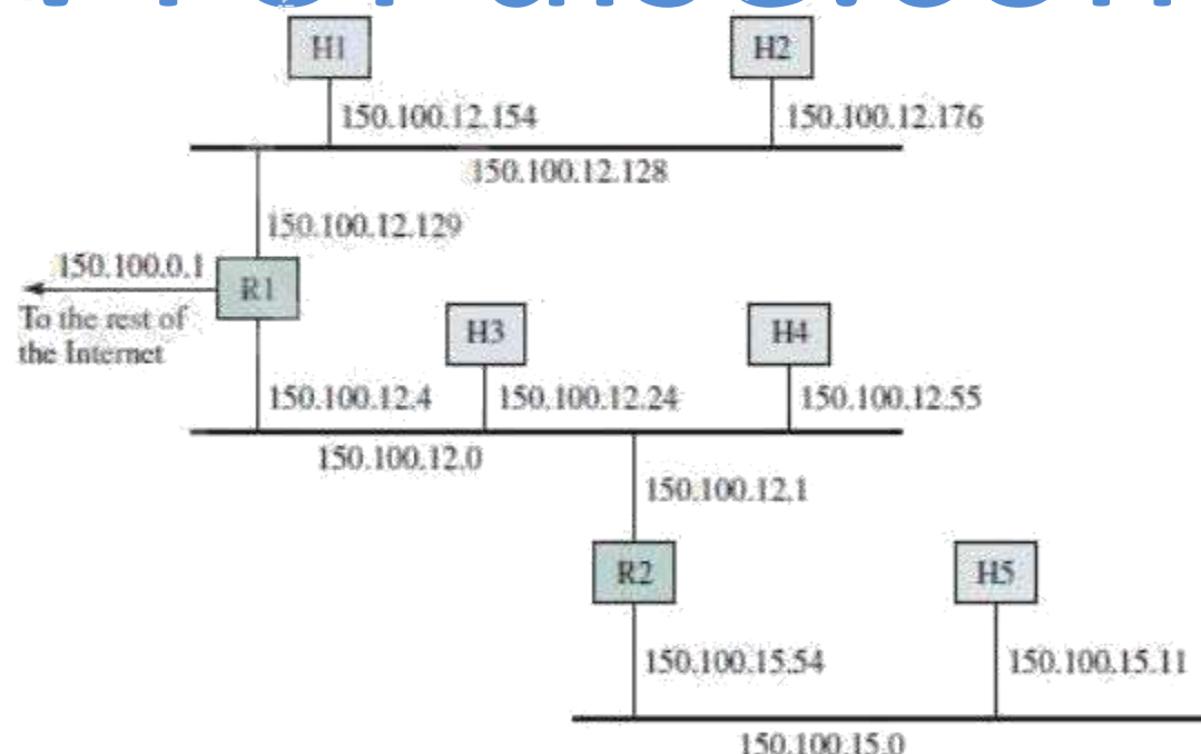
Figure 3.15: Example of address assignment with subnetting
