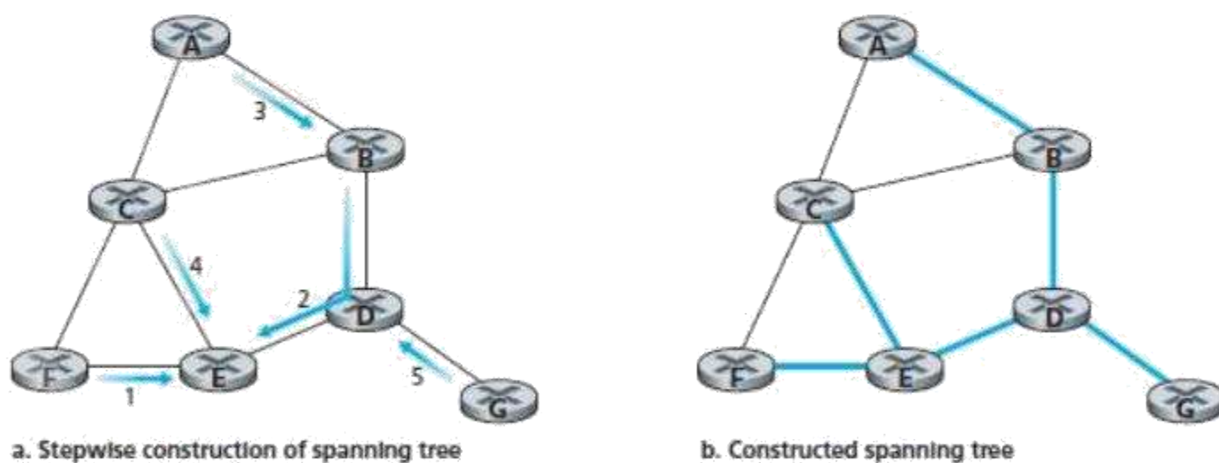
Figure 3.34: Center-based construction of a spanning-tree
