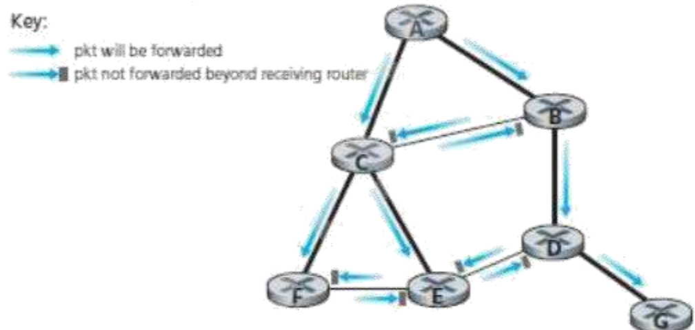
Figure 3.32: Reverse path forwarding
