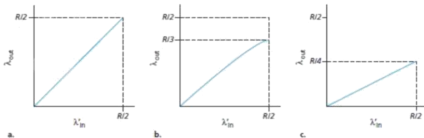
Figure 2.38: Scenario 2 performance with finite buffers
