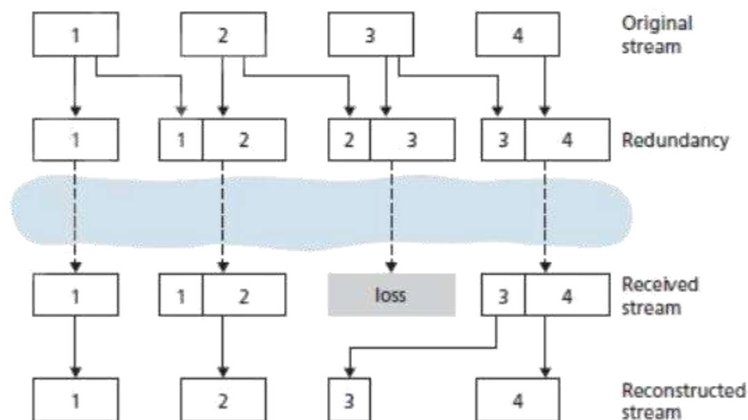
Figure 5.4: Piggybacking lower-quality redundant information
