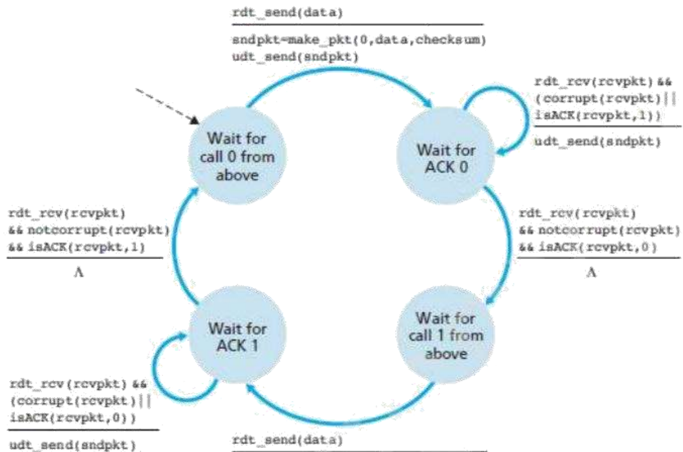
Figure 2.12: rdt2.2 sender
