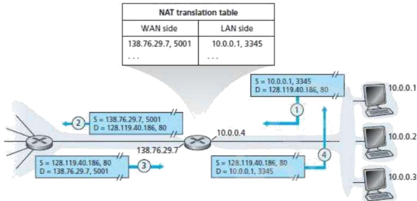
Figure 3.17: Network address translation
