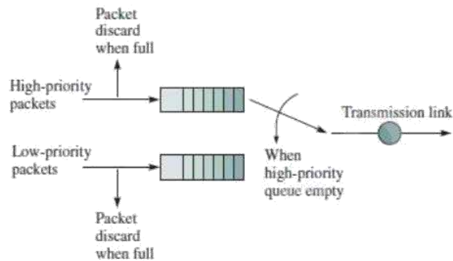
Figure 5.14 : Priority Queueing
