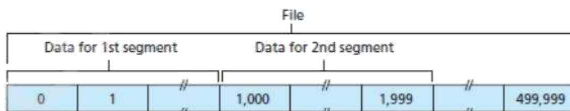
Figure 2.26: Dividing file data into TCP segments
