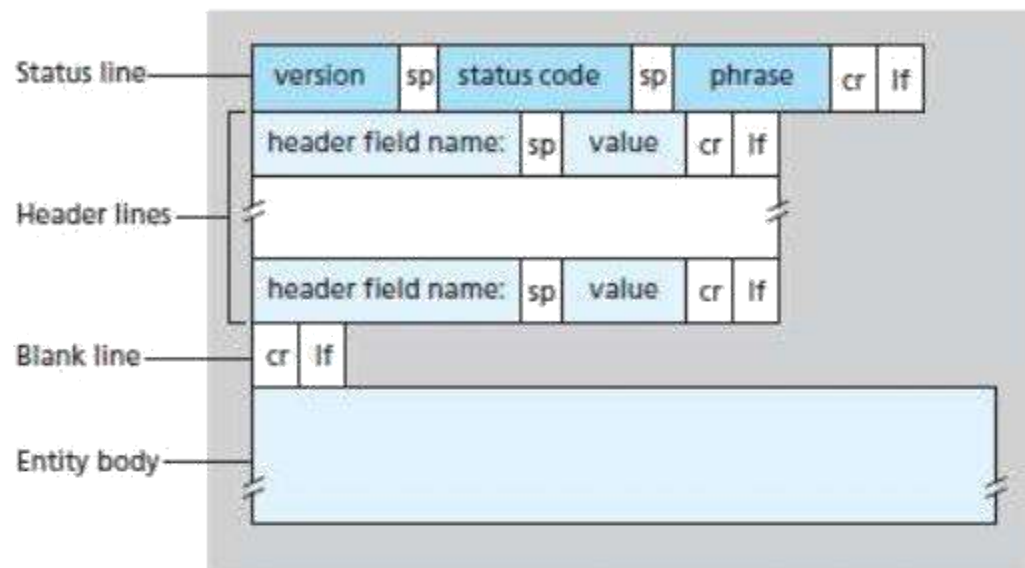
Figure 1.6: General format of an HTTP response-message
