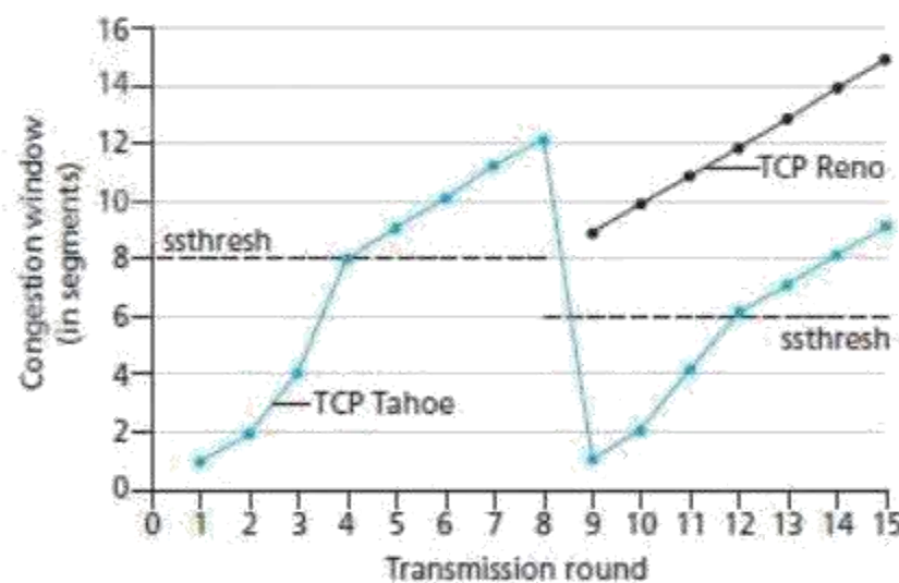
Figure 2.44: Evolution of TCP's congestion-window (Tahoe and Reno)
