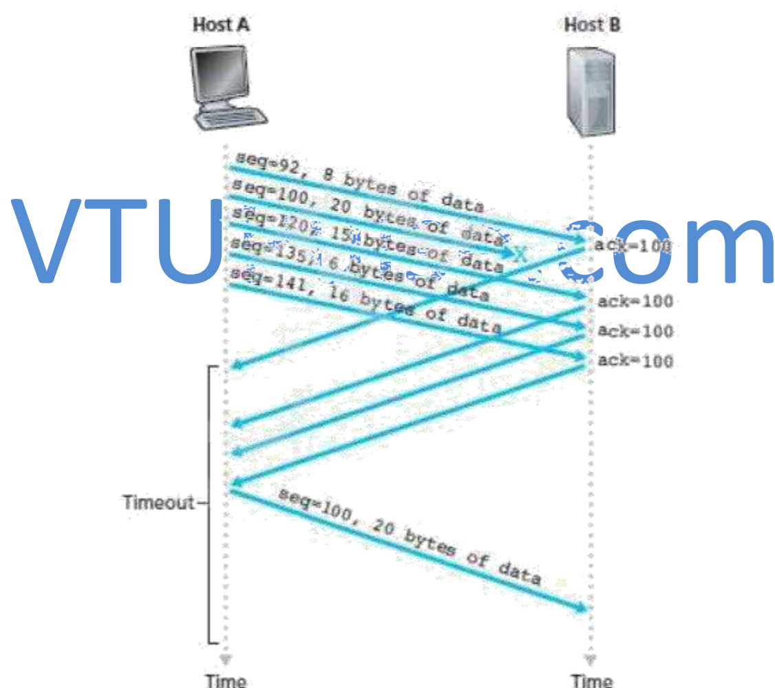
Figure 2.31: Fast retransmit: retransmitting the missing segment before the segment's timer expires
