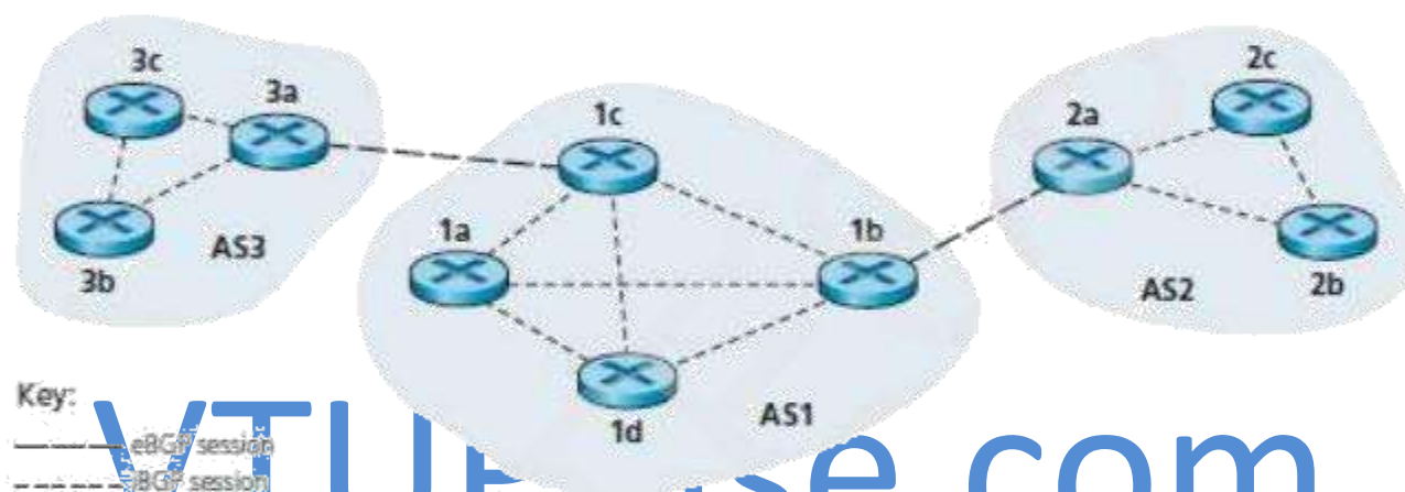
Figure 3.29: eBGP and iBGP sessions
