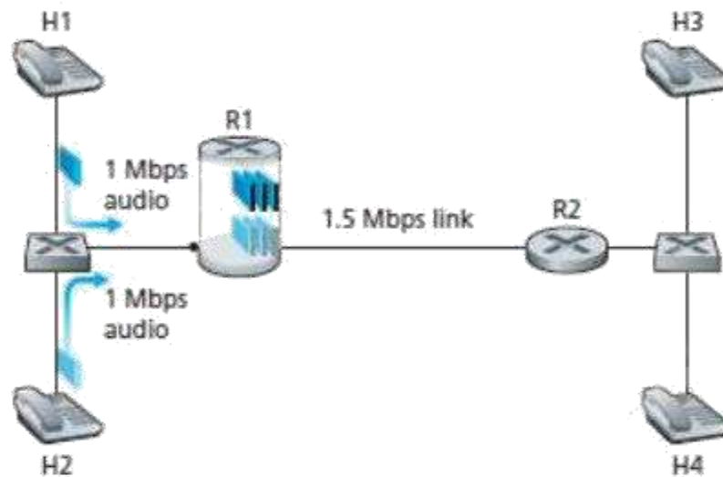
Figure 5.22: Two competing audio applications overloading R1-to-R2 link
