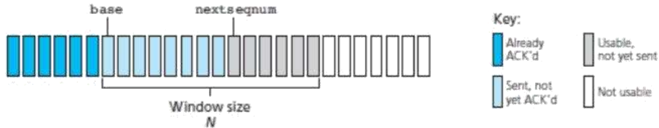
Figure 2.17: Sender's view of sequence-numbers in Go-Back-N
