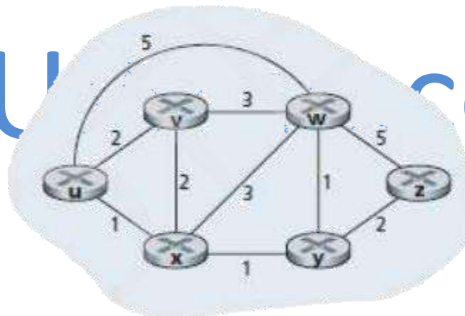
Figure 3.22: Abstract graph model of a computer network
