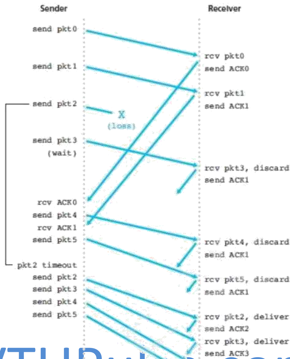
Figure 2.20: Go-Back-N in operation
