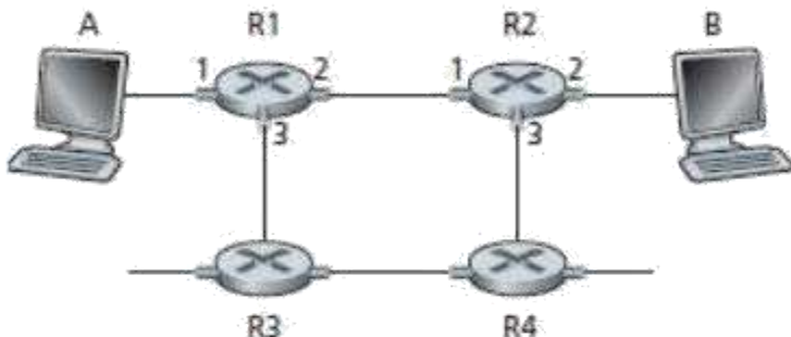
Figure 3.2: A simple virtual-circuit network
