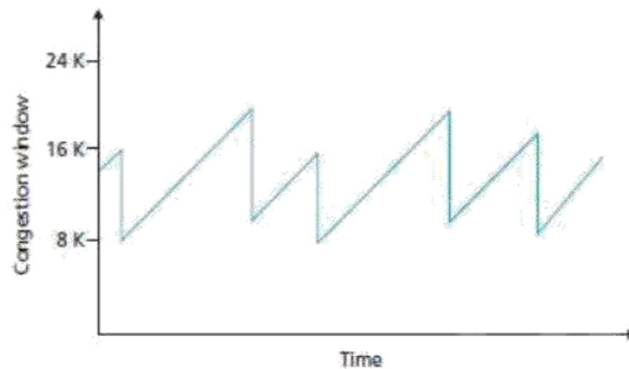
Figure 2.45: Additive-increase, multiplicative-decrease congestion-control
