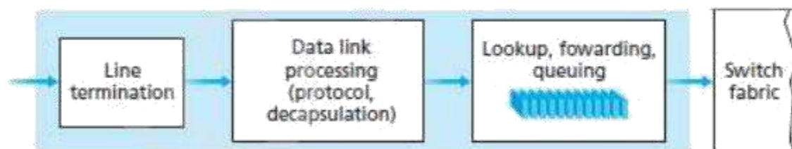
Figure 3.6: Input port processing
