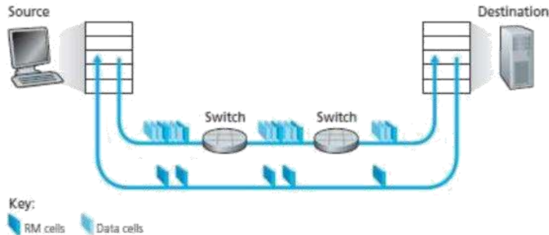
Figure 2.41: Congestion-control framework for ATM ABR service
