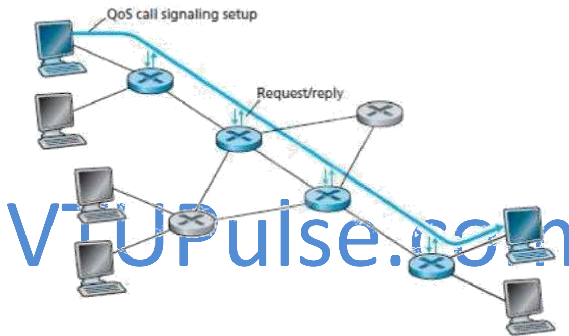
Figure 5.23: The call setup process
