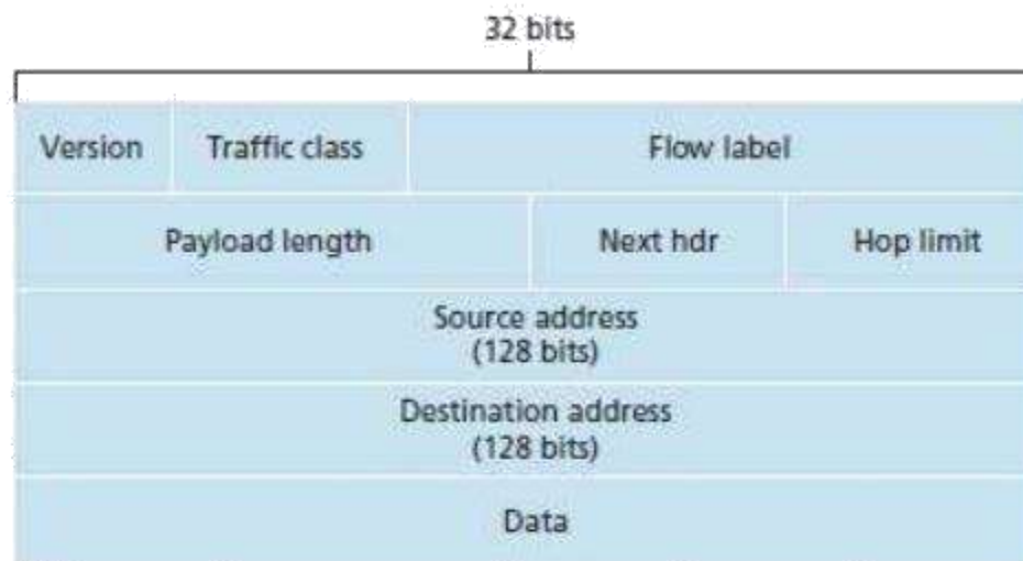
Figure 3.18: IPv6 datagram format
