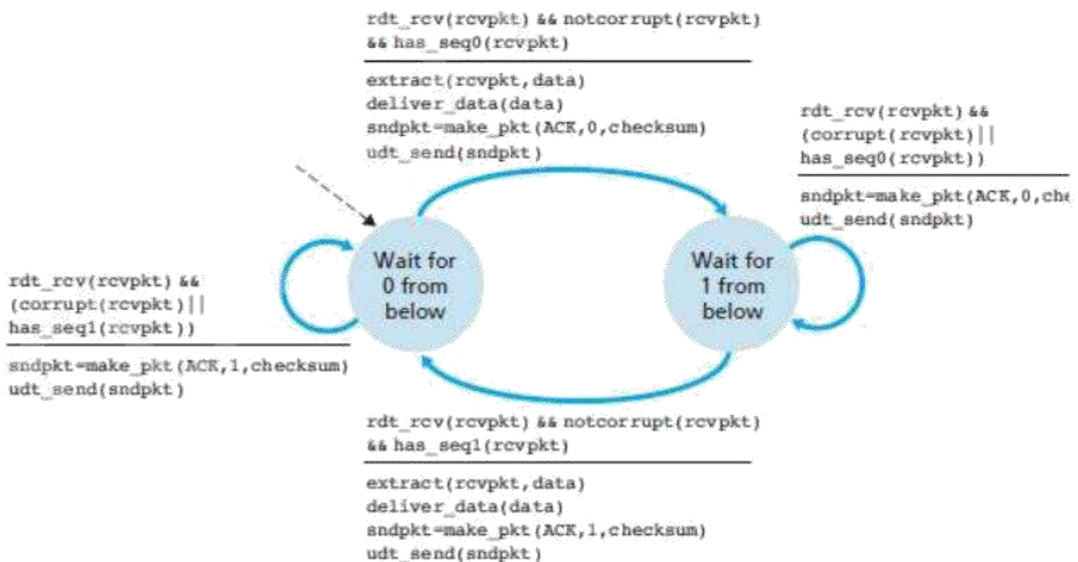
Figure 2.13: rdt2.2 receiver
