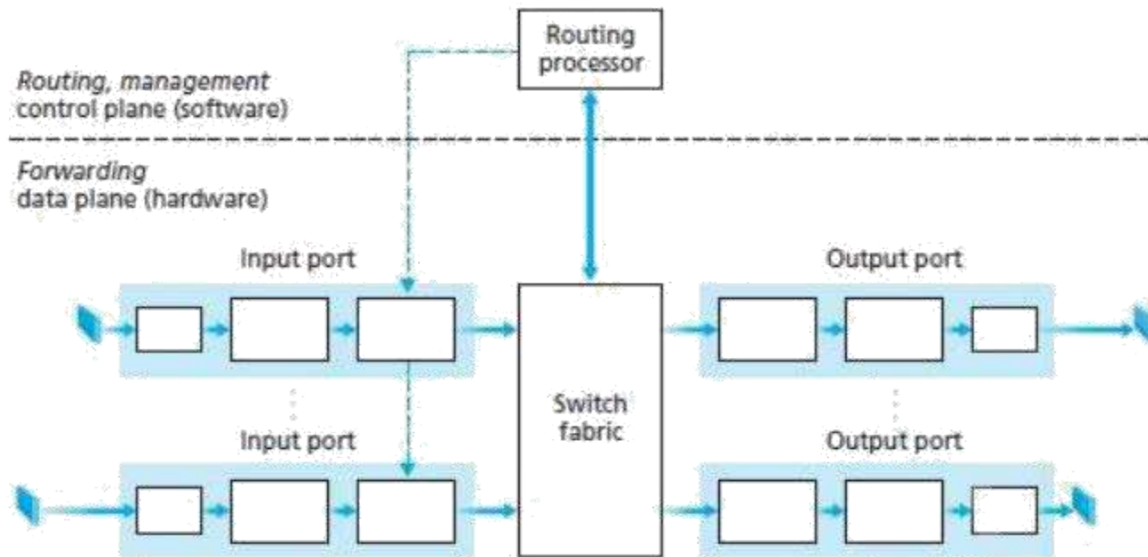
Figure 3.5: Router architecture
