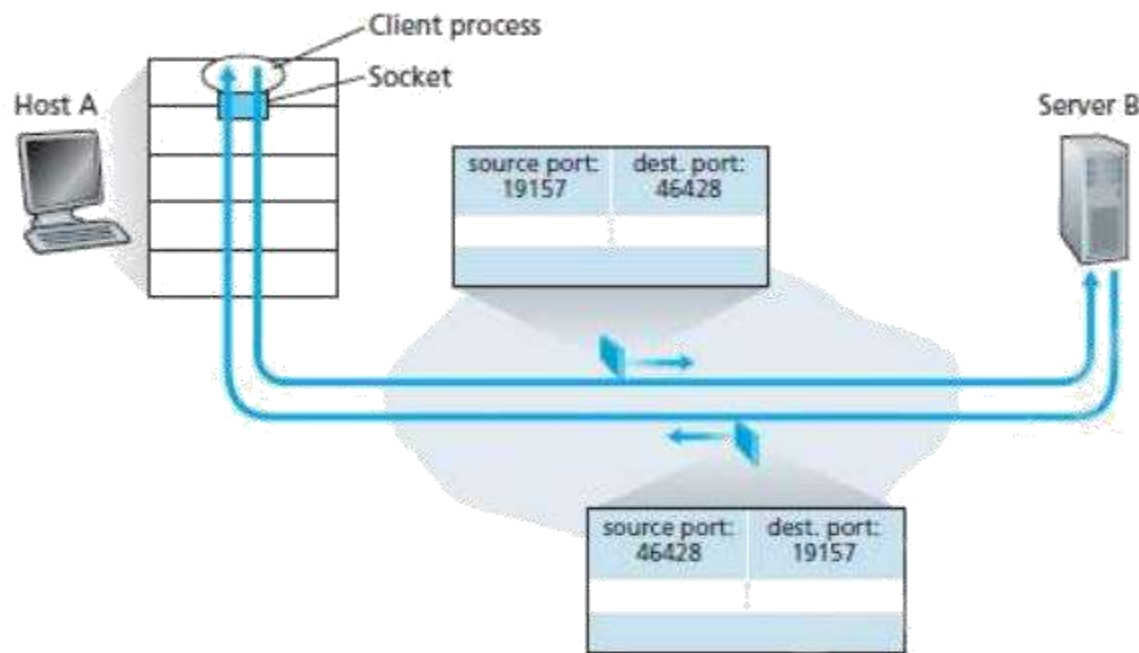
Figure 2.3: The inversion of source and destination-port-nos
