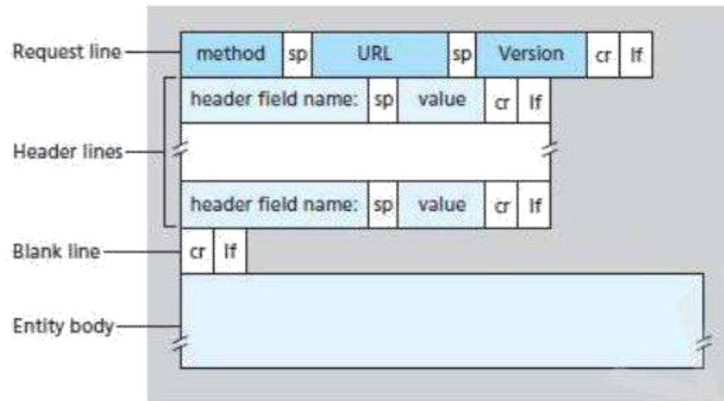
Figure 1.5: General format of an HTTP request-message
