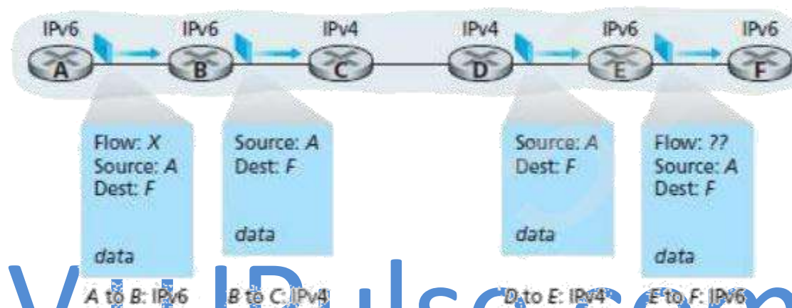
Figure 3.20: A dual-stack approach
