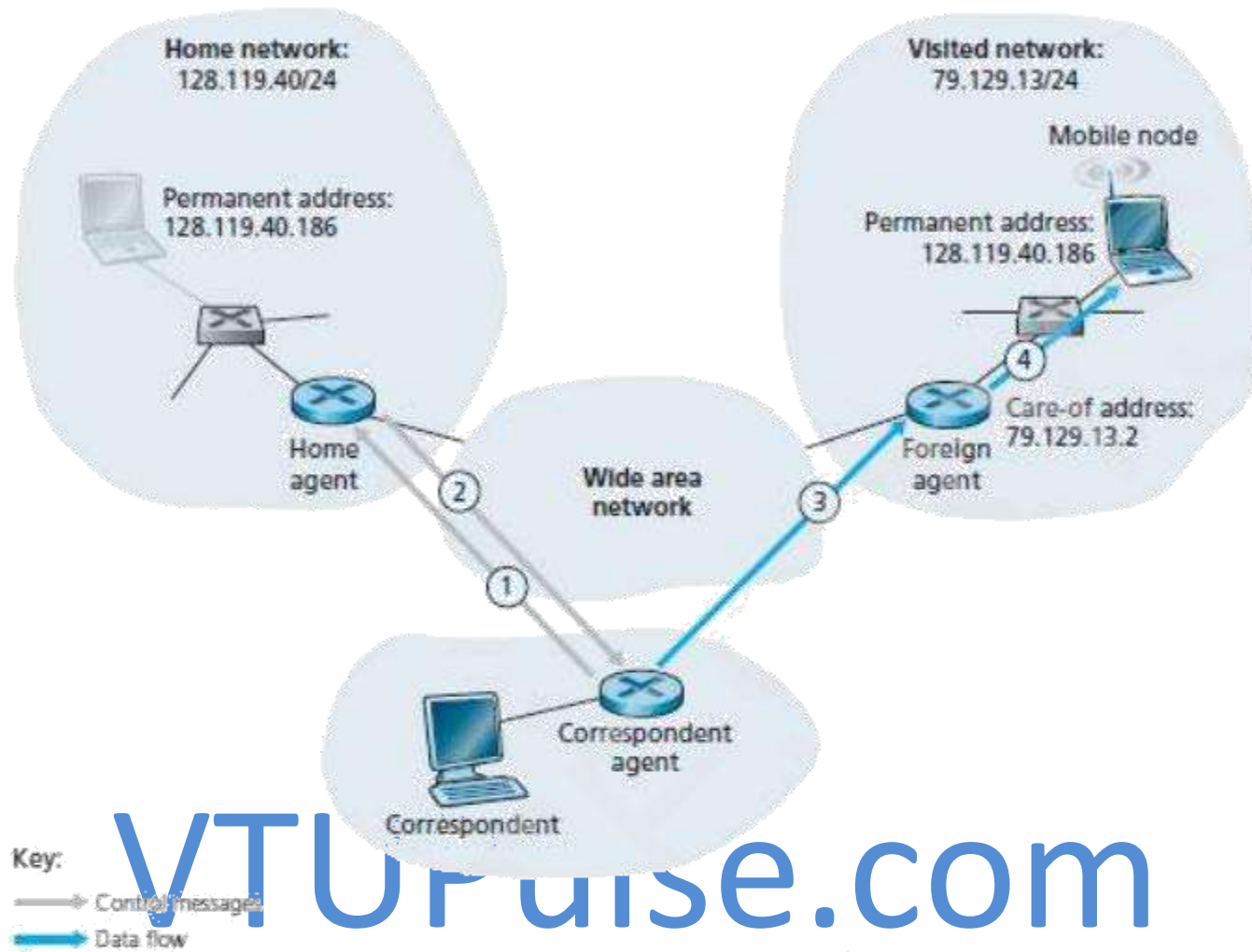
Figure 4.6: Direct routing to a mobile user
