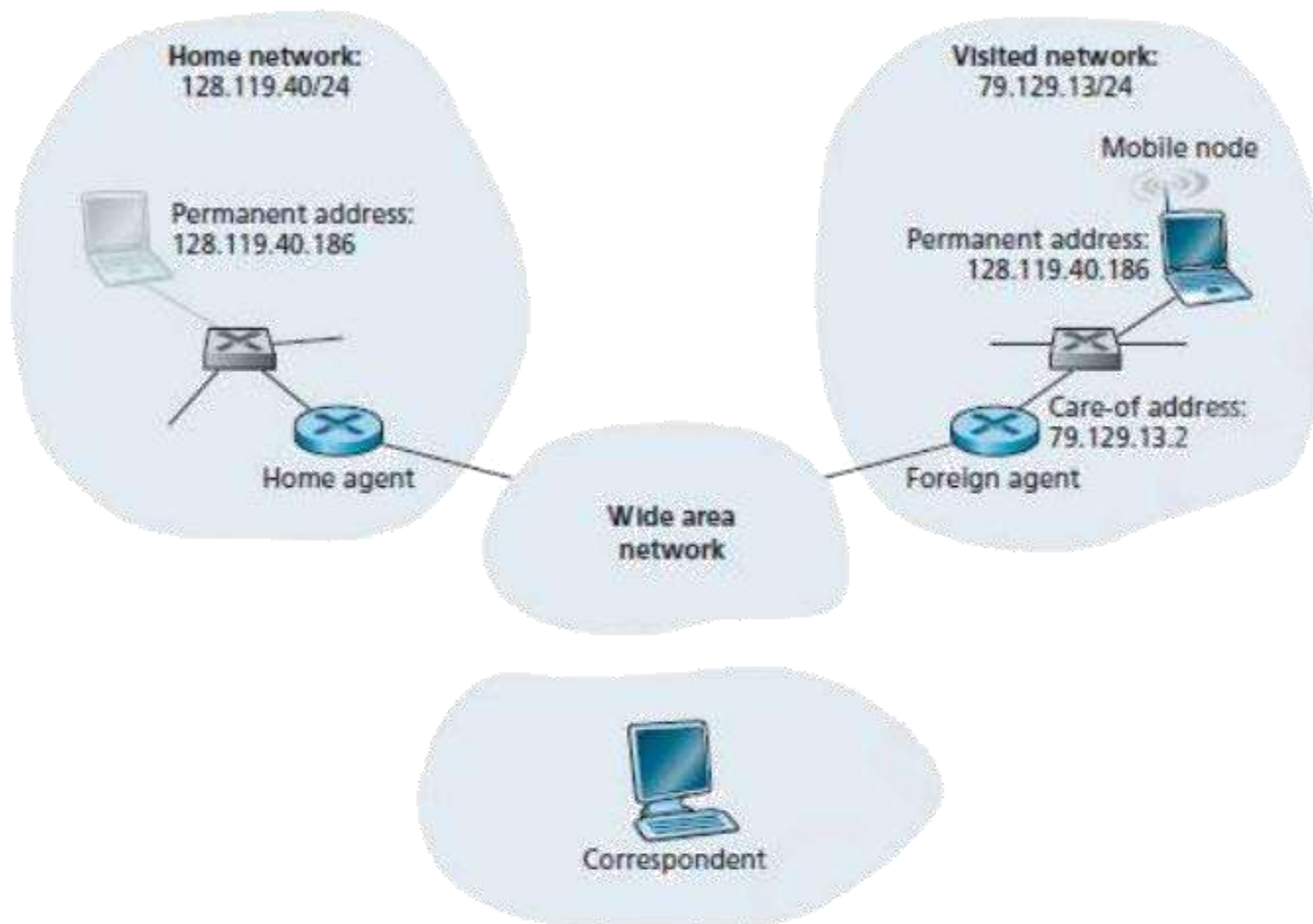
Figure 4.4: Initial elements of a mobile network architecture
