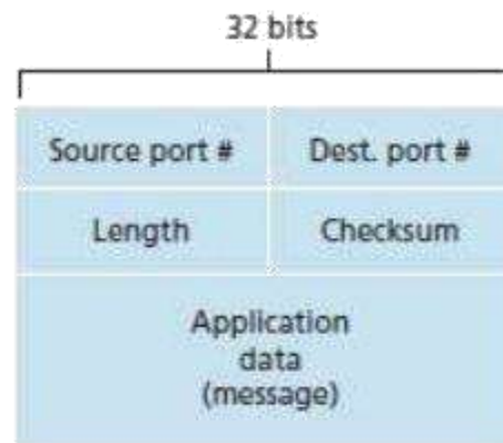
Figure 2.6: UDP segment structure
