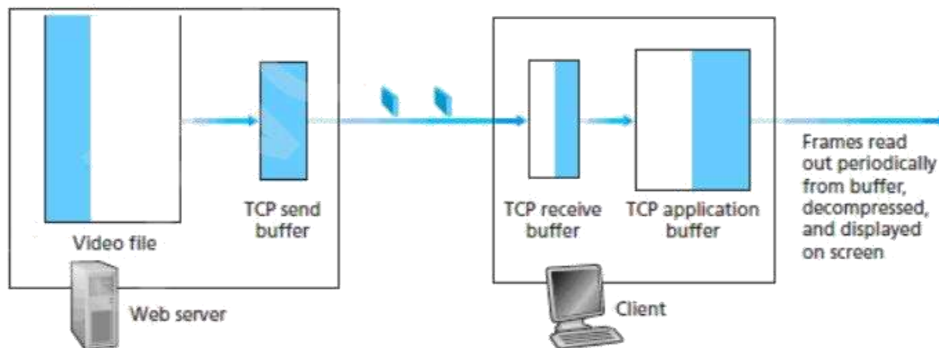
Figure 5.1: Streaming stored video over HTTP/TCP
