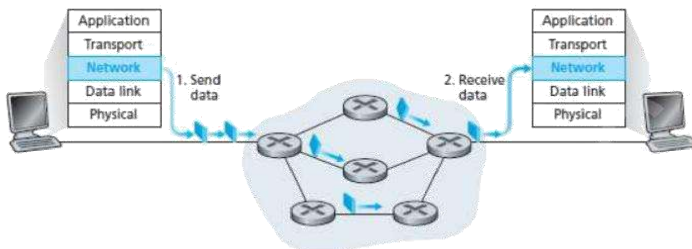
Figure 3.4: Datagram network
