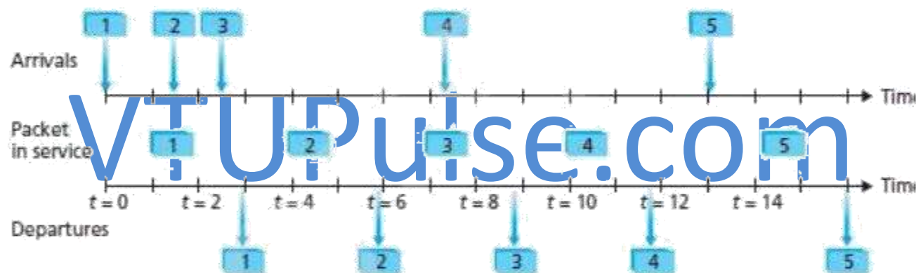
Figure 5.13: Operation of the FIFO queue
