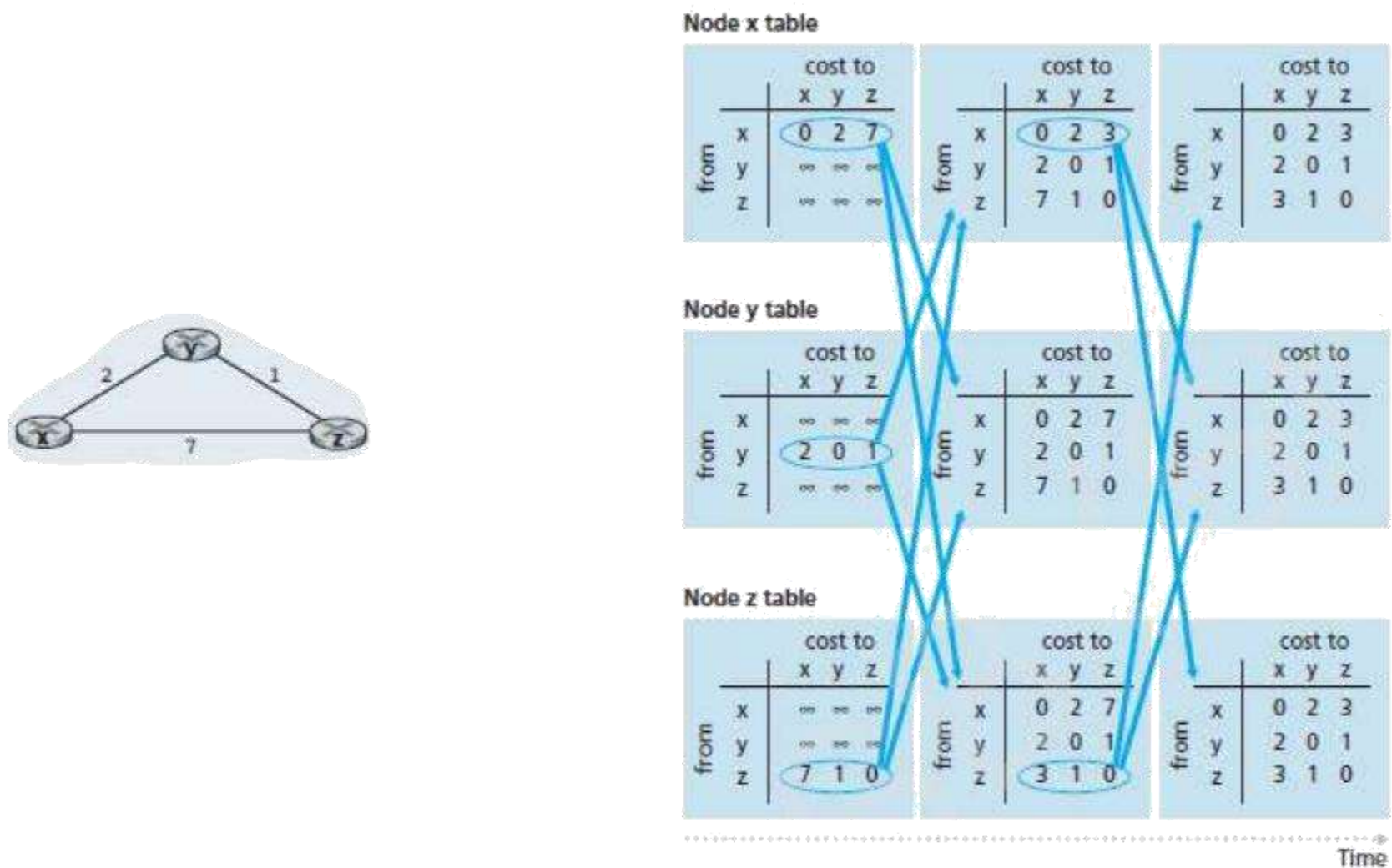
Figure 3.24: Distance-vector (DV) algorithm
