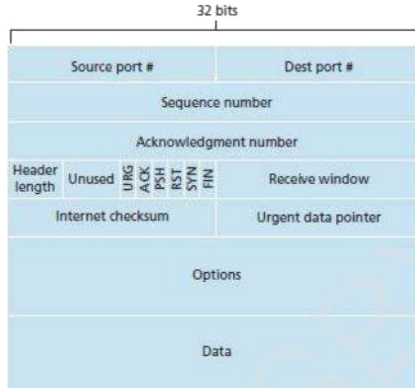
Figure 2.24: TCP segment structure
