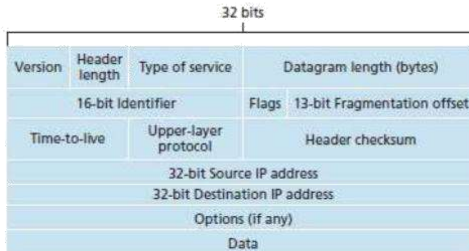
Figure 3.11: IPv4 datagram format
