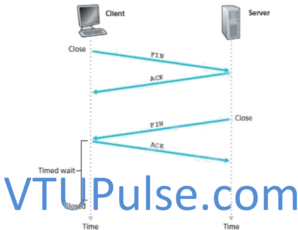
Figure 2.34: Closing a TCP connection
