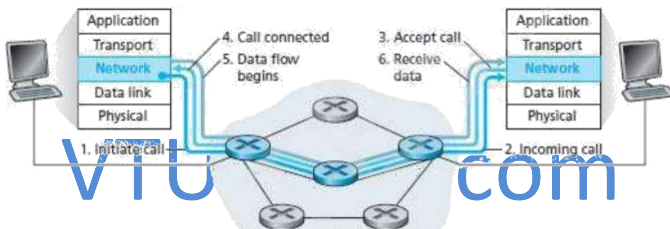
Figure 3.3: Virtual-circuit setup
