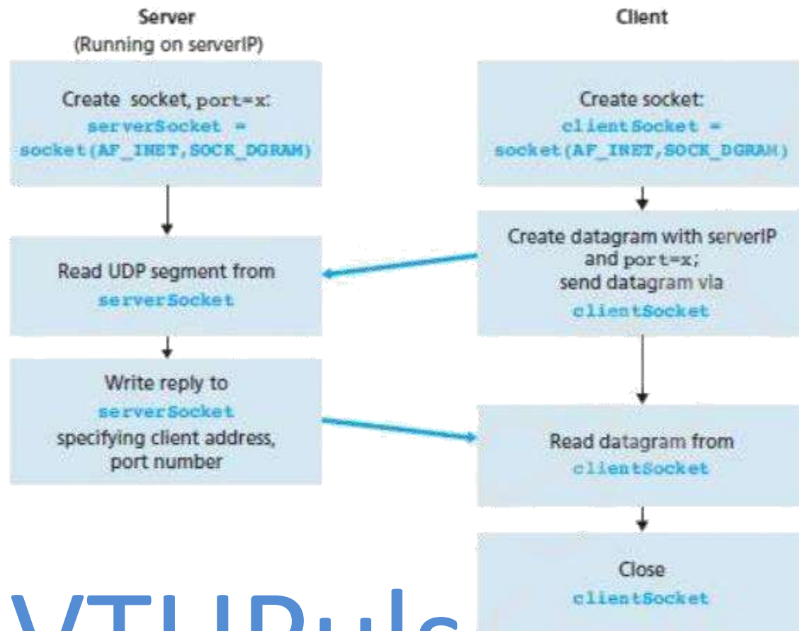
Figure 1.19: The client-server application using UDP
