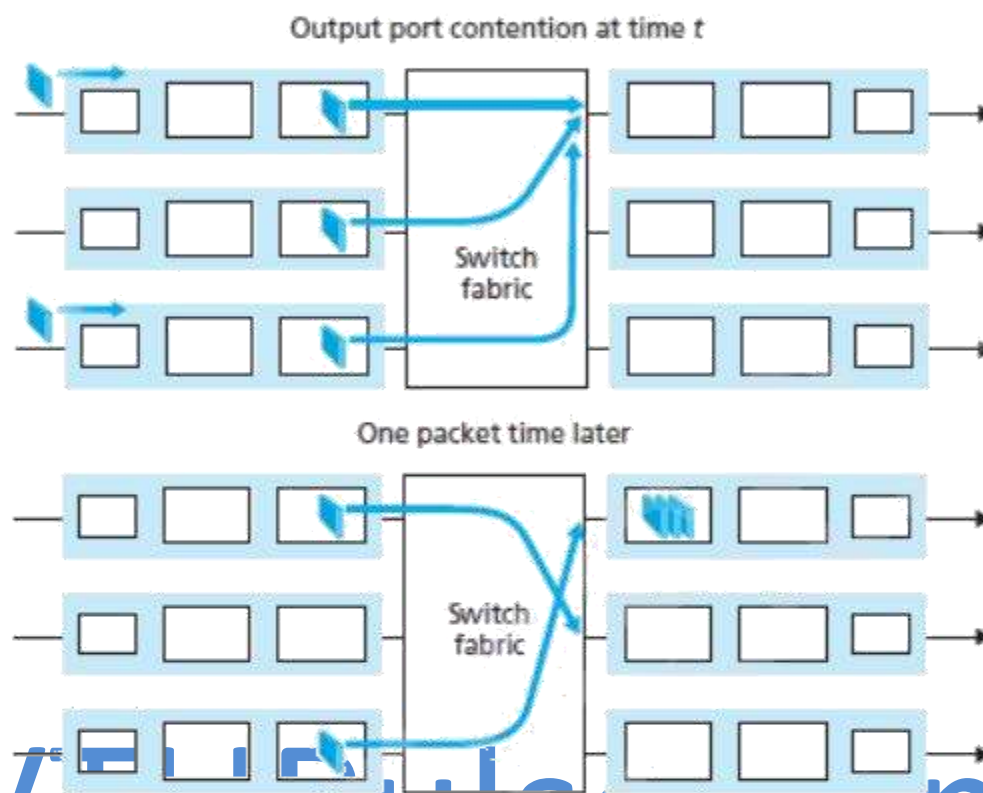
Figure 3.9: Output port queueing
