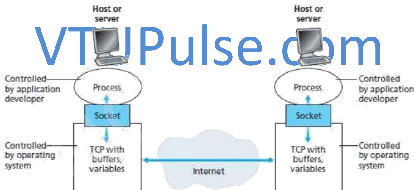
Figure 1.2: Application processes, sockets, and transport-protocol
