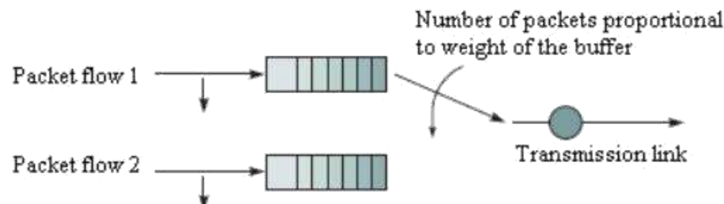
Figure 5.18: Weighted fair queuing
