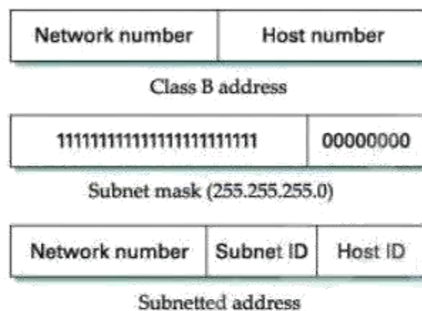
Figure 3.14: Subnet addressing
