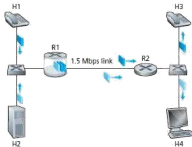
Figure 5.9: Competing audio and HTTP applications
