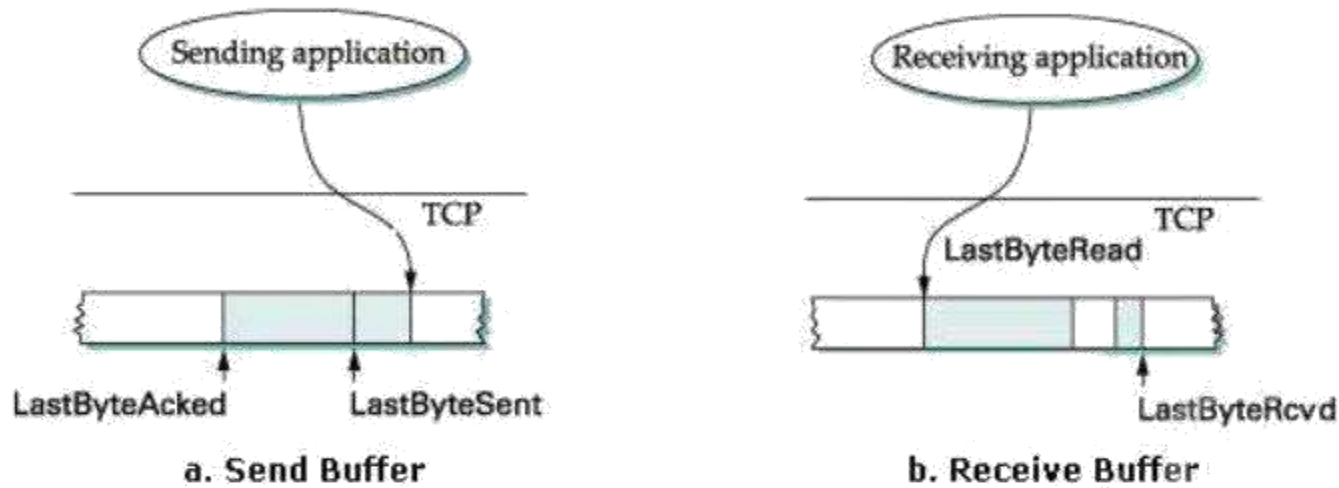
Figure 2.32: a) Send buffer and b) Receive Buffer
