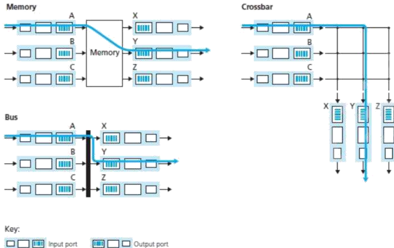
Figure 3.7: Three switching techniques
