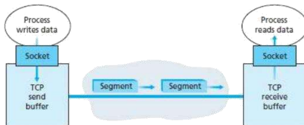
Figure 2.23: TCP send and receive-buffers
