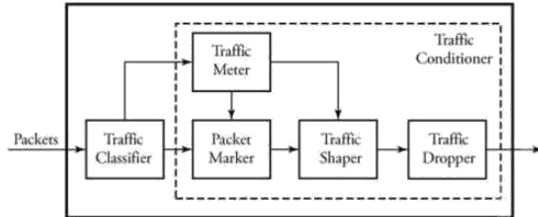
Figure 5.21: Overview of DiffServ operation
