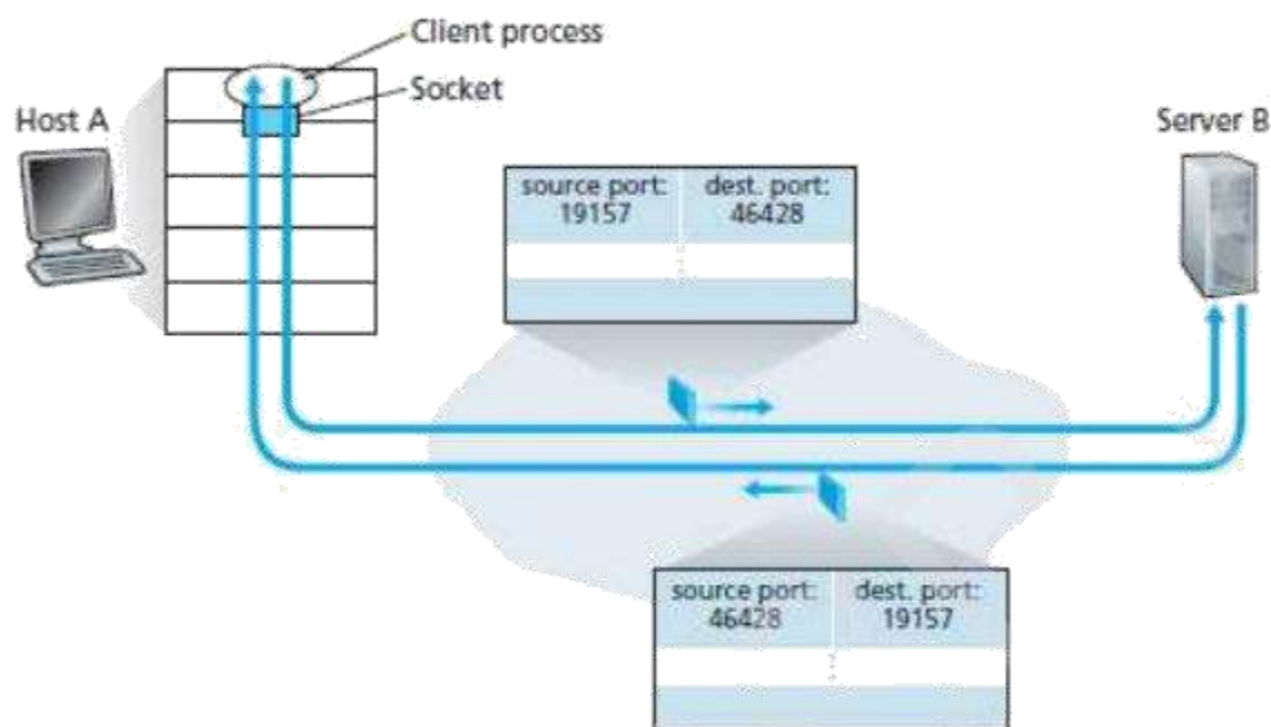
Figure 2.4: The inversion of source and destination-port-nos
