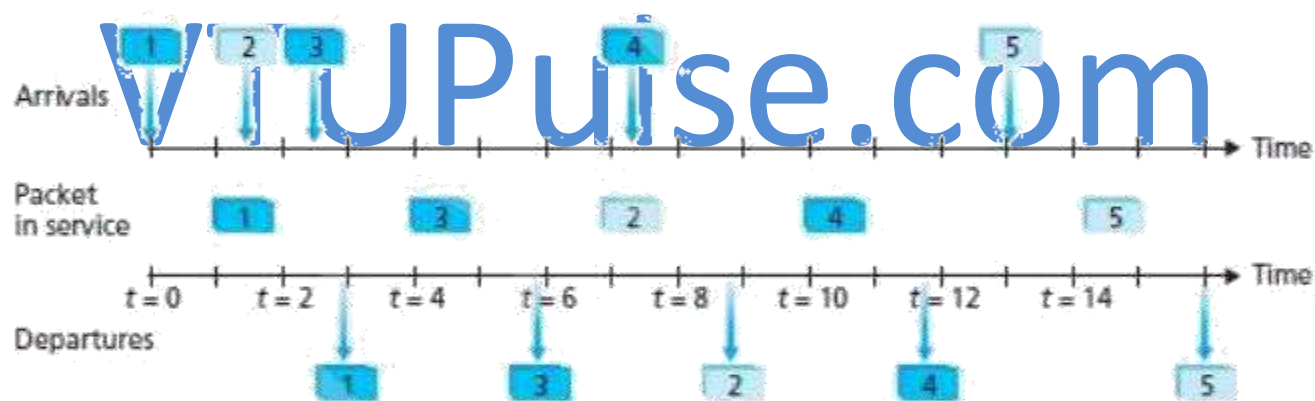
Figure 5.15: Operation of the priority queue
