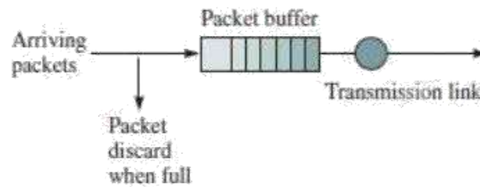
Figure 5.12: FIFO queueing
