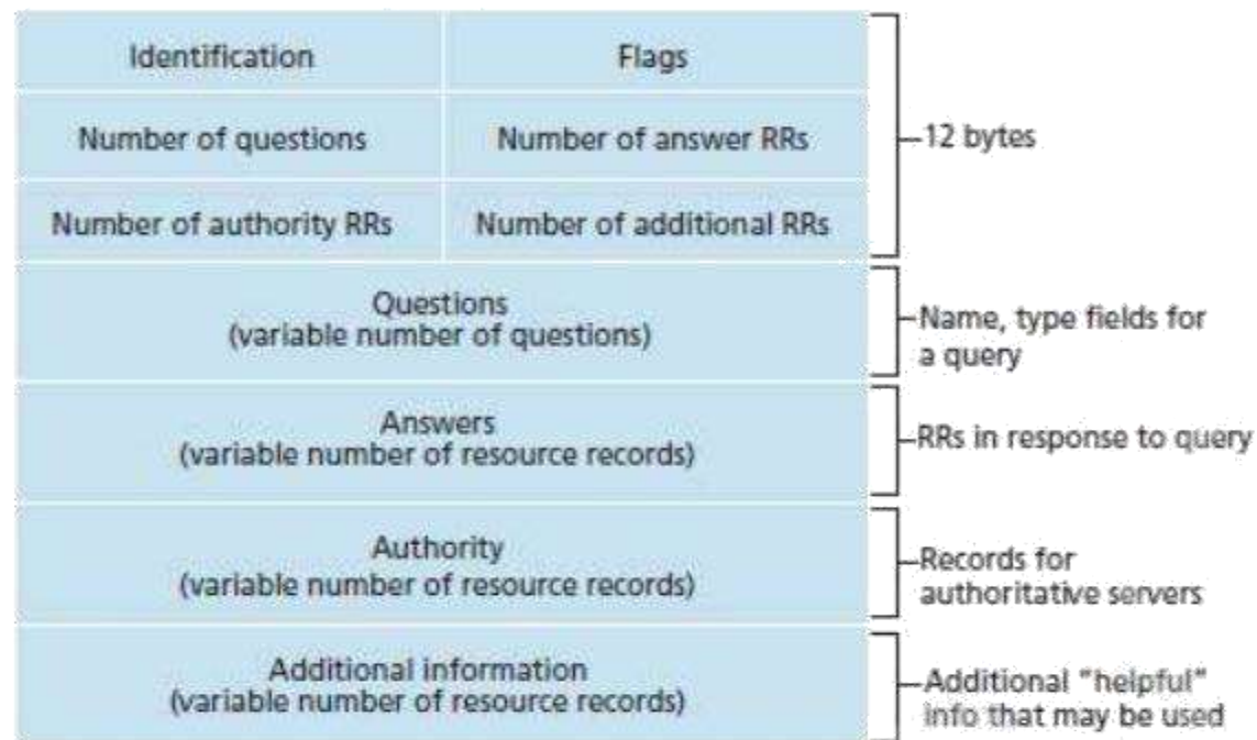
Figure 1.14: DNS message format
